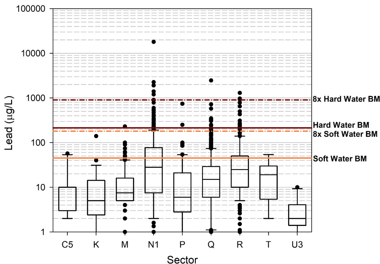
FIGURE D-10 Lead results from NetDMR 2015 MSGP reported data through February 2018. Orange lines denote the soft-water benchmark of 45 \mu\text{g/L} and hard-water benchmark of 213 \mu\text{g/L} , although benchmark exceedance is assessed based on site-specific water quality data.
