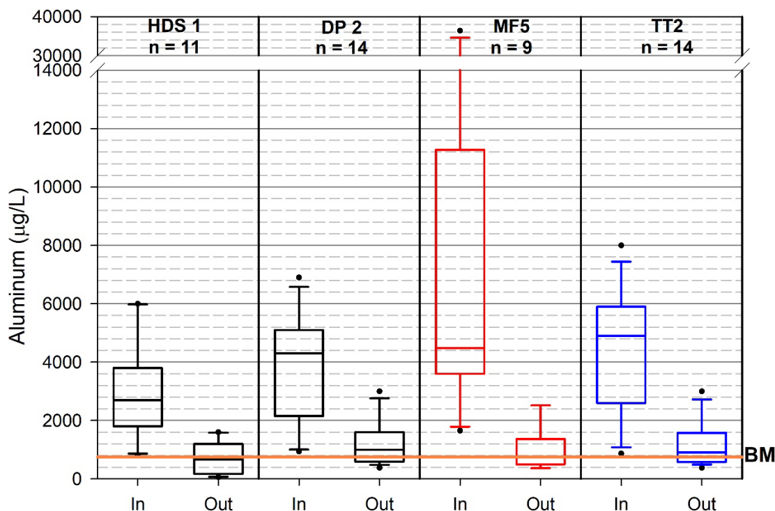
FIGURE E-1 Total aluminum influent versus effluent concentrations. DP = dry detention pond; HDS = hydrodynamic separator;; MF = media filter; TT = treatment train. The number of storm-event samples used in each analysis is shown on the graph below each treatment system.
