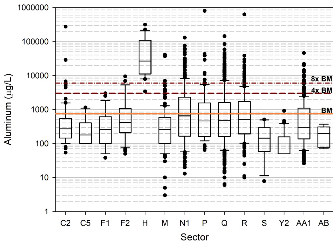
FIGURE D-1 Aluminum results from NetDMR 2015 MSGP reported results through February 2018. Orange line denotes benchmark of 750 µg/L.
