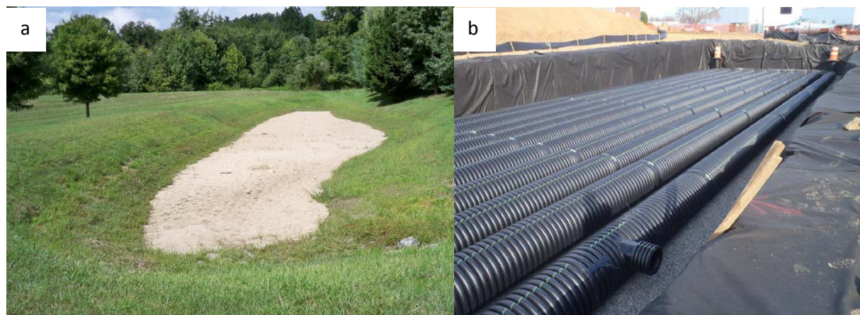
FIGURE 4-1 Aboveground (a) and belowground (b) stormwater retention facilities with infiltration. SOURCES: (a) Montgomery County Department of Environmental Protection; (b) Philadelphia Water Department.
