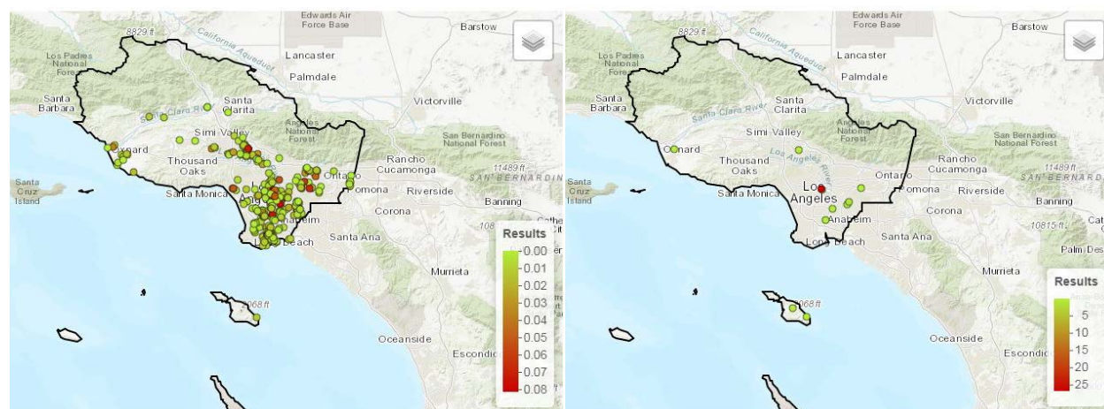
FIGURE 3-1 Median lead concentrations at sites in California Water Board, Los Angeles Region, from monitoring from the past 5 years, with results less than (left) and greater than (right) the benchmark of 82 µg/L.
