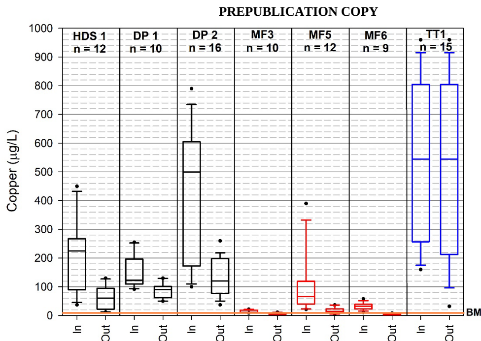
FIGURE E-3 Total copper influent versus effluent concentrations compared to the soft-water benchmark concentration of 9 \mu\text{g/L} . DP = dry retention pond; HDS = hydrodynamic separator; MF = media filter; TT = treatment train. The number of storm-event samples used in each analysis is shown on the graph below each treatment system.
