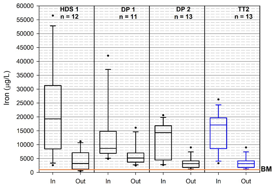
FIGURE 2-3 Total iron influent versus effluent concentrations comparison at industrial sites from Clark and Pitt (in press).
