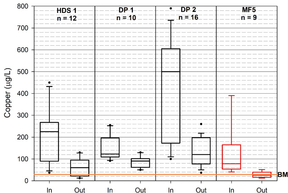
FIGURE E-4 Total copper influent versus effluent concentrations compared to the hard-water benchmark concentration of 28.5 \mu\text{g/L} . DP = dry retention pond; HDS = hydrodynamic separator; MF = media filter. The number of storm-event samples used in each analysis is shown on the graph below each treatment system.
