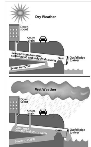
Figure 3. Schematic of a typical combined sewer system that discharges, directly to surface waters during wet weather. Source: EPA
